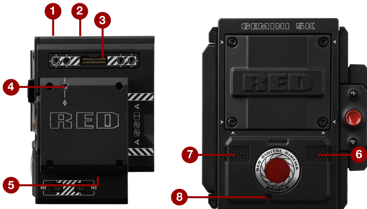
Figure: DSMC2 GEMINI Ports and Features
