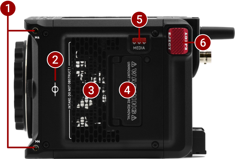
Figure: Camera Body Left Controls and Features
